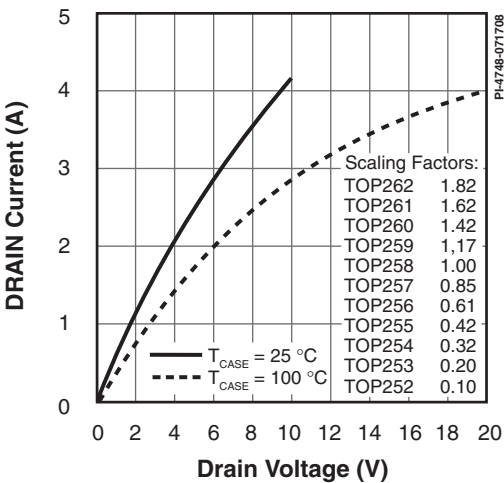
Figure 66. Output Characteristics.
