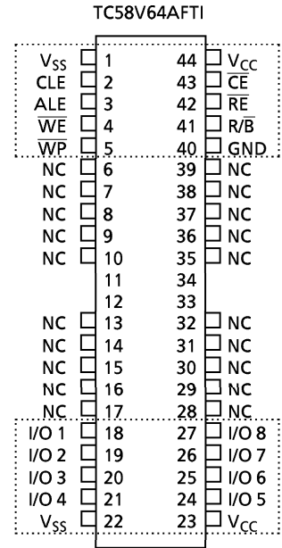
Figure 1. Pinout
