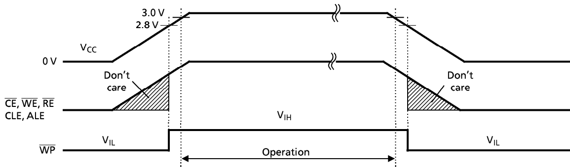
Figure 21. Power-on/off Sequence
