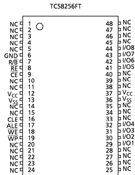
Figure 1. Pinout
