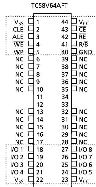
Figure 1. Pinout
