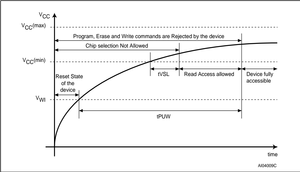
Figure 20. Power-up timing
