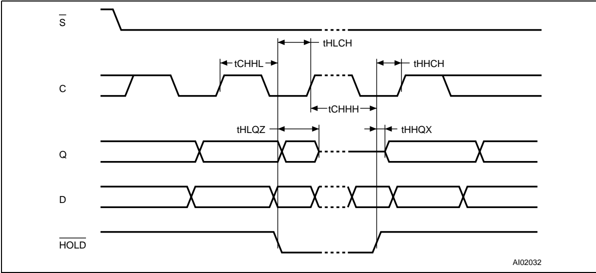
Figure 24. Hold timing
