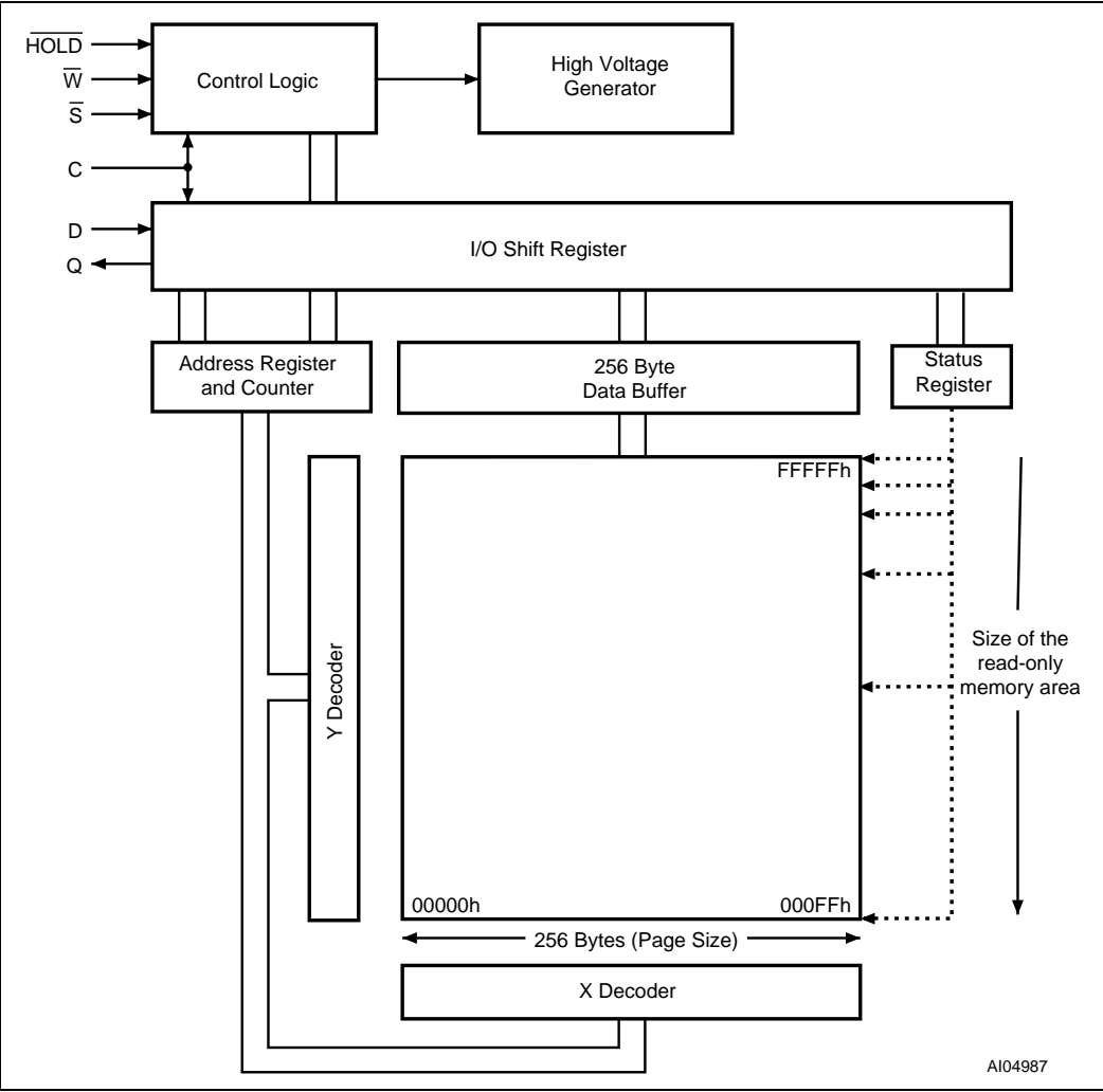
Figure 6. Block diagram
