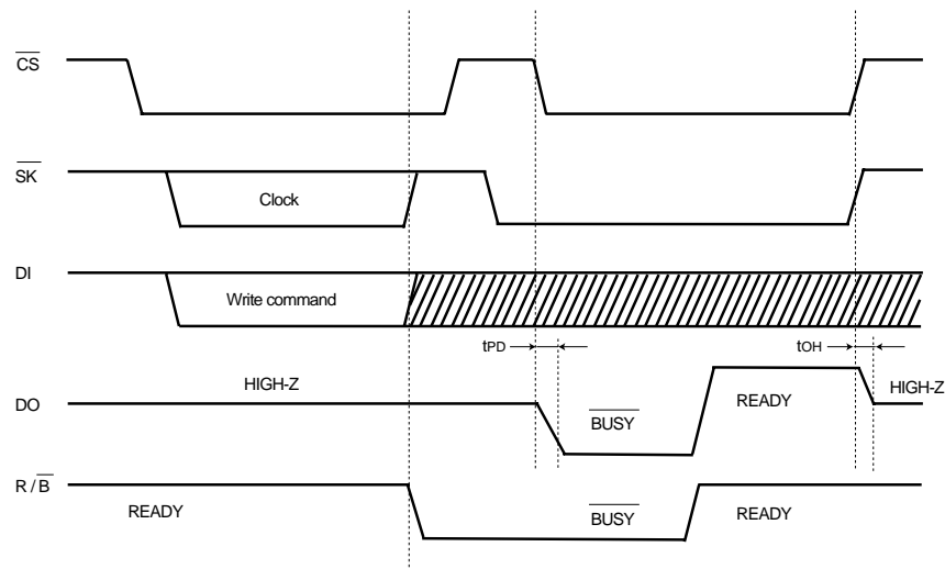
Fig.8 \overline{\text{R}} / \overline{\text{B}} Status Output timing chart
