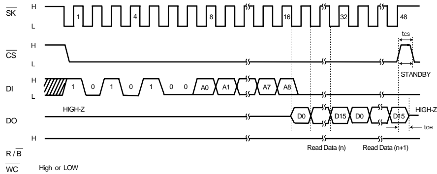
Fig.4 BR9080AF-W / ARFV-W / ARFVM-W
