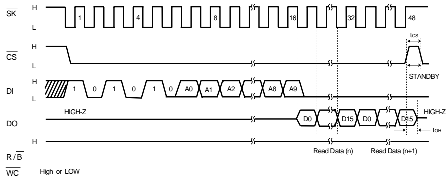
Fig.5 BR9016AF-W / ARFV-W / ARFVM-W
