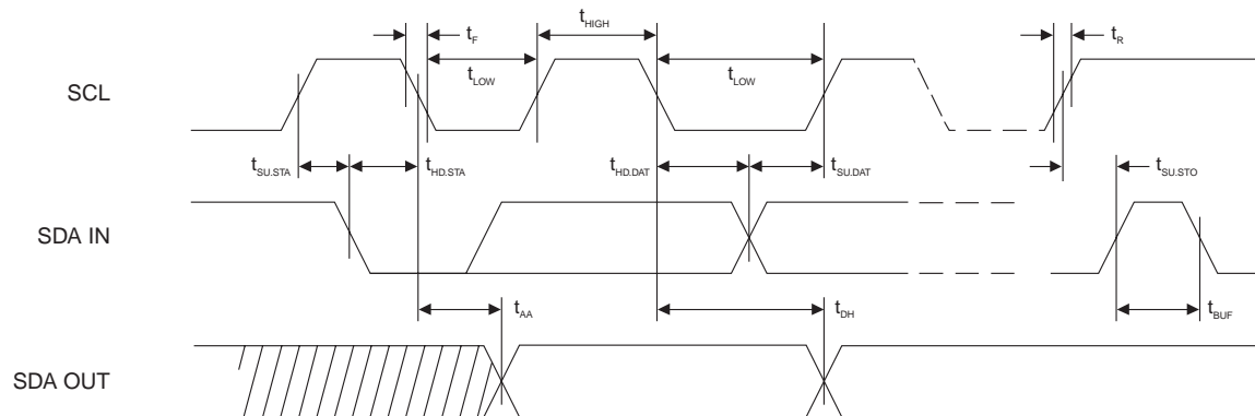
Figure 4-4. Bus Timing
