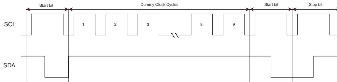
Figure 4-3. Software Reset
