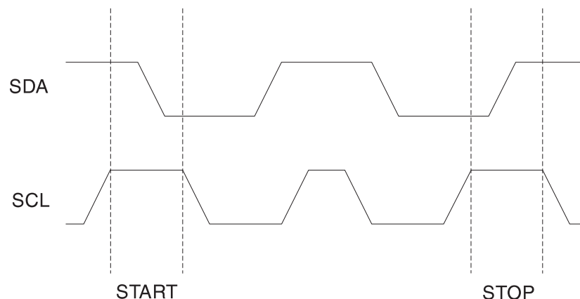
Figure 10-1. Start and Stop Definition
