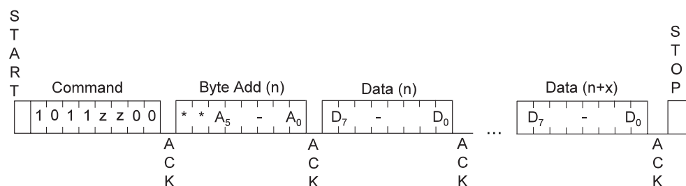
Figure 9-2. Write EEPROM
