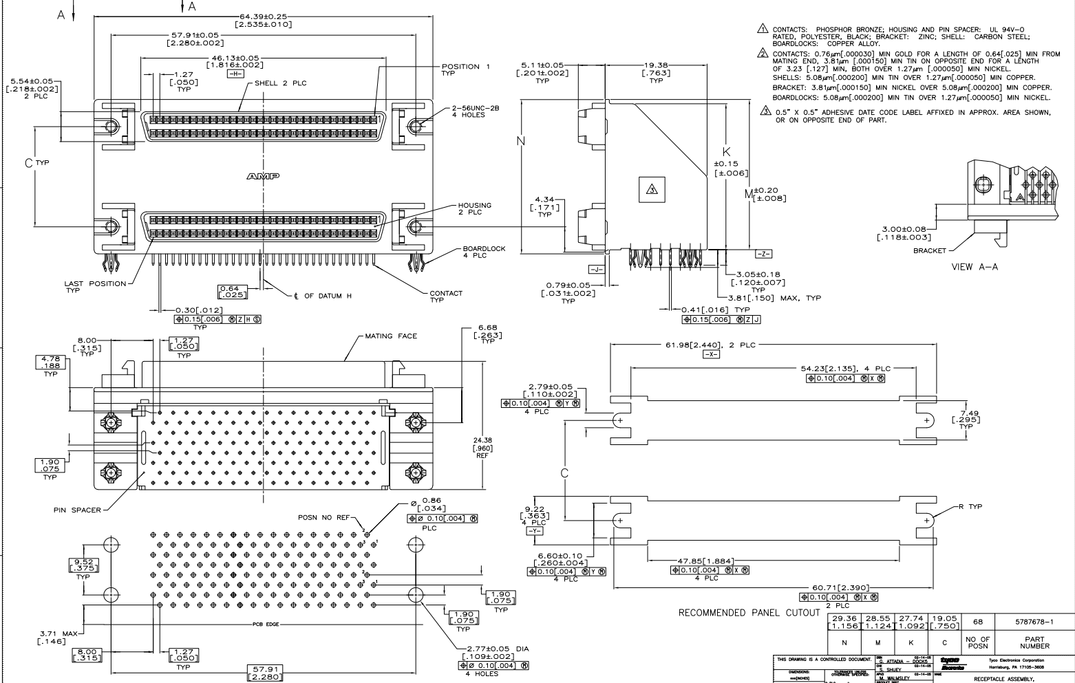
RECOMMENDED P.C. BOARD MOUNTING DIMENSIONS CONNECTOR SIDE P.C. BOARD THICKNESS: 1.57±0.20 [.062±.008]
