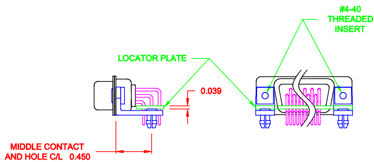
BRACKETS MOUNTED ON CONNECTOR WITH LOCATOR PLATE
