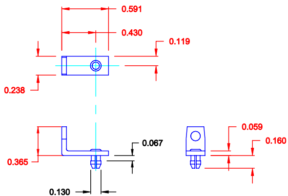
MOUNTING BRACKET WITH BOARD LOCK
