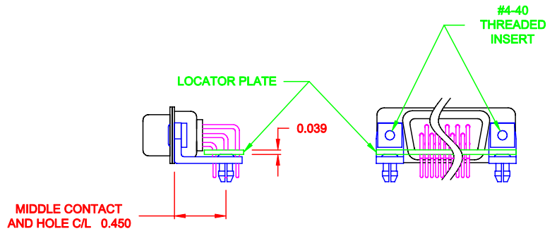
BRACKETS MOUNTED ON CONNECTOR WITH LOCATOR PLATE
