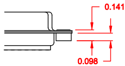
01X ..... 0.098" (BOARD SIDE) - CN1
