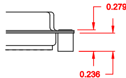
02X ..... 0.236" (BOARD SIDE) - CN2
