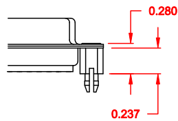
05X ..... 0.237" (BOARD SIDE) - CN10
