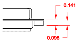
01X ..... 0.098" (BOARD SIDE) - CN1
