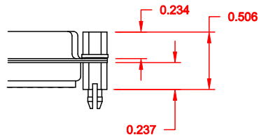
91X ..... 0.237" BOARD SIDE 0.197 MATING SIDE CN10/SFSO4404
