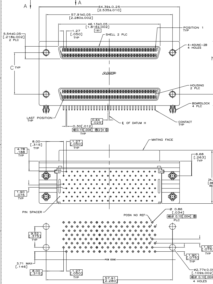
RECOMMENDED P.C.BOARD MOUNTING DIMENSIONS CONNECTOR SIDE P.C.BOARD THICKNESS 1.57±0.20 [.062±0.008]
