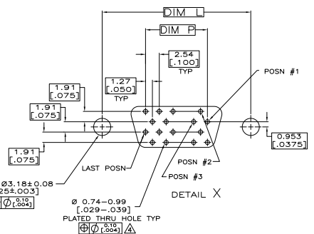
P.C.BOARD MOUNTING DIMENSIONS (CONNECTOR SIDE)
