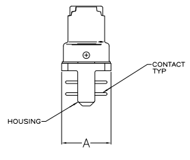
TERMINATED VIEW
