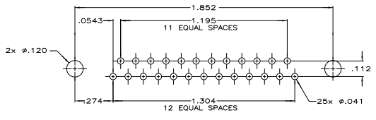
RECOMMENDED P.C. BOARD MOUNTING DIMENSIONS △
