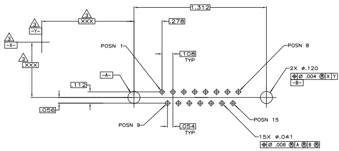
RECOMMENDED PC BOARD MOUNTING DIMENSIONS
