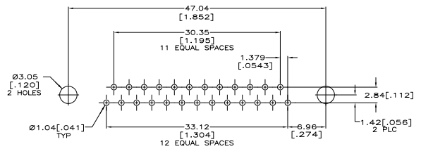
RECOMMENDED P.C. BOARD MOUNTING DIMENSIONS
