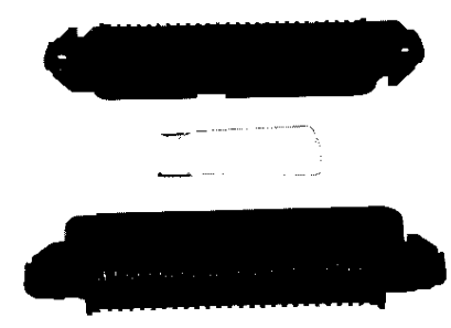
CHAMP-LOK Hardware Kit (One locking latch required per assembly) Part No. 552723-1 (36 or 50 Pos. Locking Latch) Part No. 552723-2 (14 or 24 Pos. Locking Latch) Part No. 552723-3 (64 Pos. Locking Latch)
