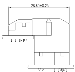
RIGHT ANGLE PLUG ASSEMBLY MATED WITH RIGHT ANGLE RECEPTACLE ASSEMBLY
