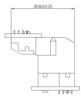
RIGHT ANGLE PLUG ASSEMBLY MATED WITH RIGHT ANGLE RECEPTACLE ASSEMBLY
