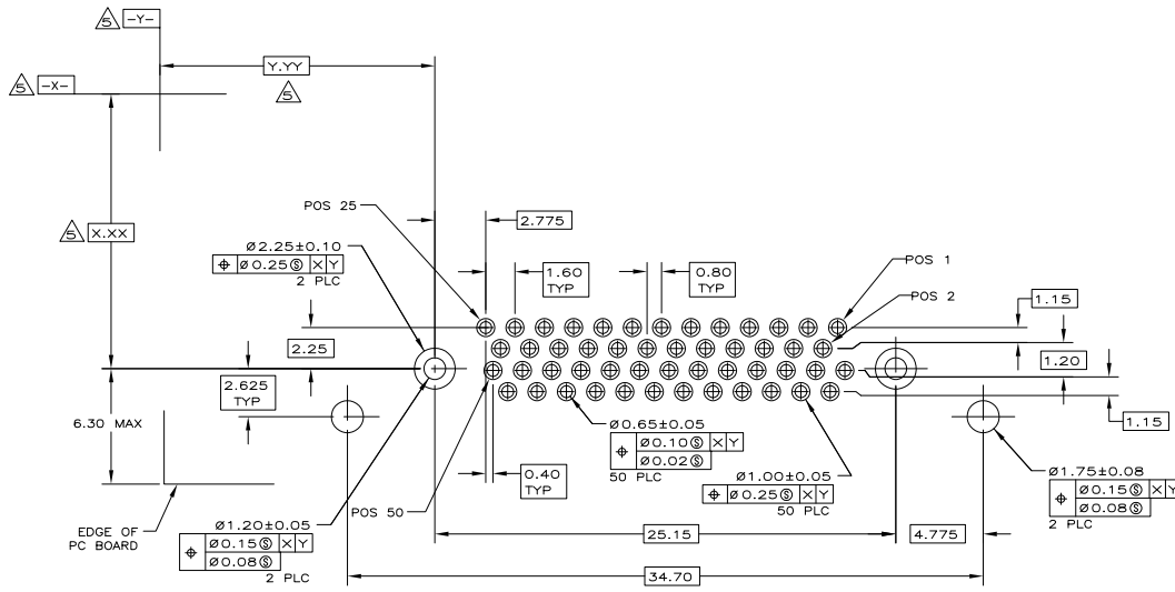
PC BOARD MOUNTING DIMENSIONS \Delta
