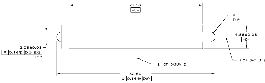
PANEL CUT-OUT DIMENSIONS \Delta
