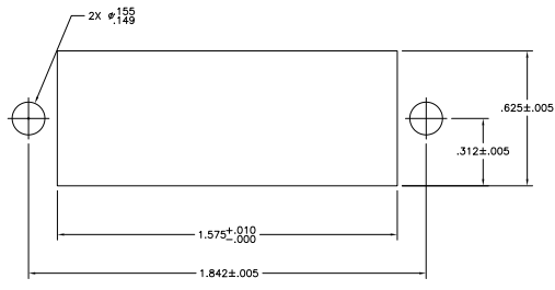
SUGGESTED REAR PANEL MOUNTING CUTOUT DIMENSION
