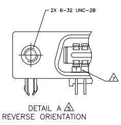
REAR PANEL MOUNTING DETAIL SHOWN FOR REFERENCE ONLY
