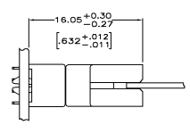
VERTICAL RECEPTACLE ASSEMBLY MATED TO VERTICAL PLUG STRADDLE ASSEMBLY
