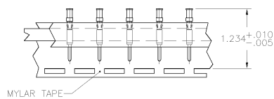
TAPE MTG. DETAIL △ 796964-2 ONLY
