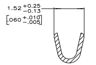
SECTION X-X INSULATION BARREL SCALE 20:1
