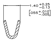
SECTION Y-Y WIRE BARREL SCALE 20:1
