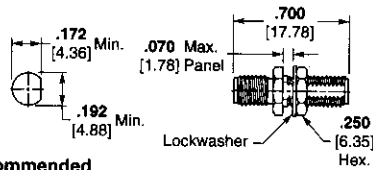
Recommended Mounting Hole
