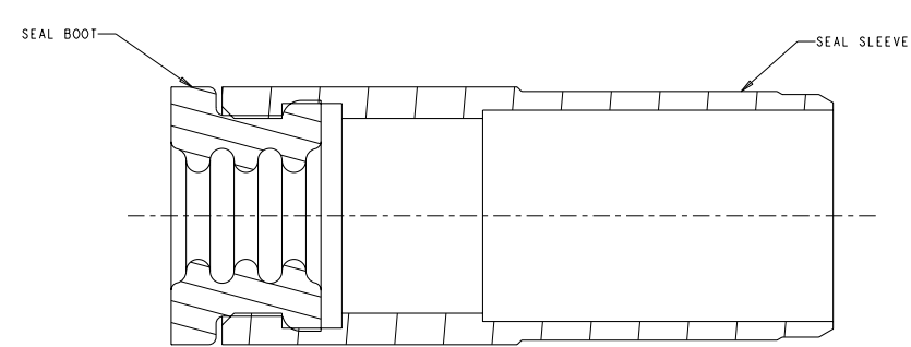
SECTION J - J
