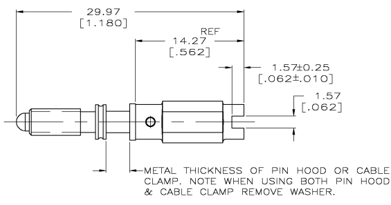
ASSEMBLED VIEW
