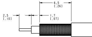
RECOMMENDED CABLE STRIPPING DIM'S. SCALE 5.000
