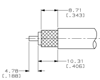
RECOMMENDED STRIP LENGTH SCALE 2:1
