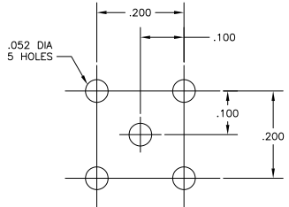
RECOMMENDED PCB HOLE CONFIGURATION
