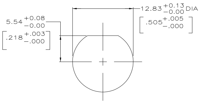
RECOMMENDED PANEL CUTOUT SCALE: 4:1
