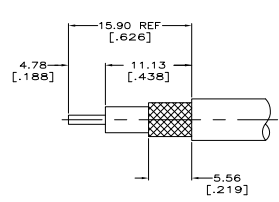
RECOMMENDED STRIP LENGTH
