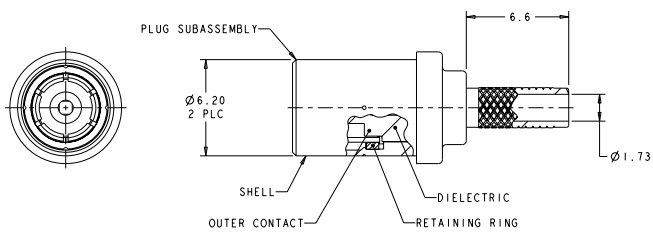
ASSEMBLED VIEWS
