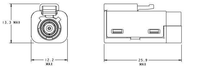
ASSEMBLED VIEWS
