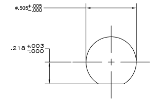
SUGGESTED PANEL CUTOUT
