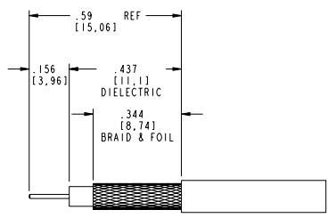
RECOMMENDED CABLE STRIPPING DIMENSIONS SCALE 3.000
