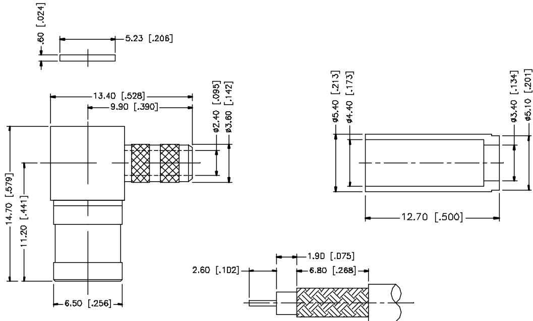
RECOMMENDED CABLE STRIPPING DIM'S
