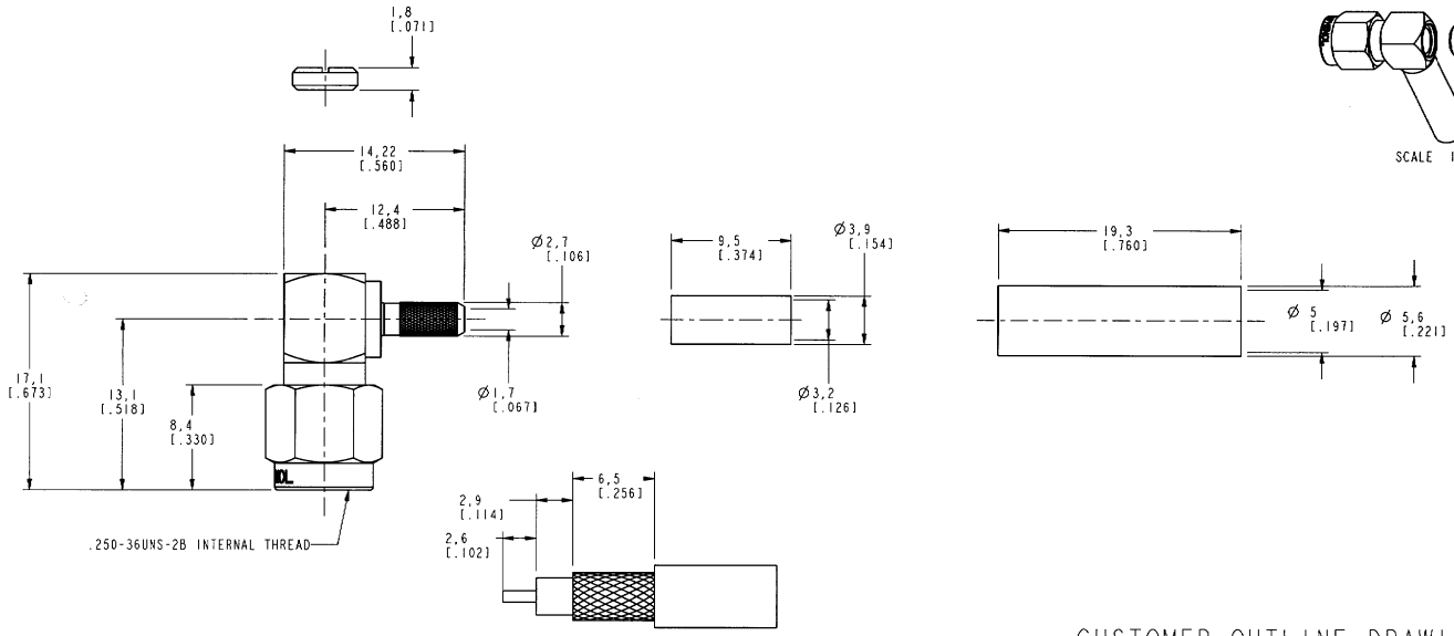
RECOMMENDED CABLE STRIPPING DIMENSIONS SCALE 3.000
