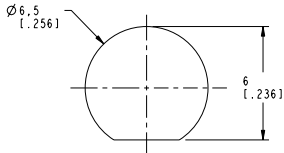
RECOMMENDED MOUNTING HOLE DIMENSIONS SCALE 5.000
