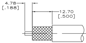
VIEW X RECOMMENDED STRIP LENGTH SCALE 2:1
