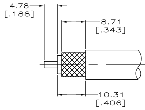
VIEW Z RECOMMENDED STRIP LENGTH SCALE 2:1
