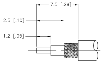
RECOMMENDED CABLE STRIP LENGTH (NTS)
