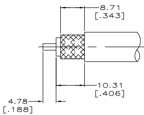
RECOMMENDED STRIP LENGTH (SCALE 2:1)
