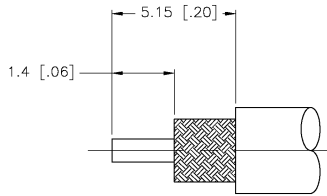
RECOMMENDED CABLE STRIP LENGTH (NTS)
