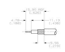
RECOMMENDED STRIP LENGTH SCALE 2:1
