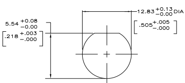
RECOMMENDED PANEL CUTOUT
