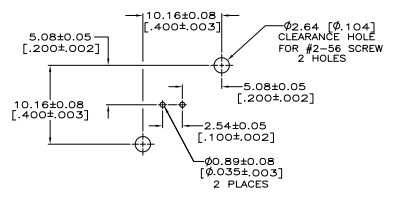
PCB CONFIGURATION
