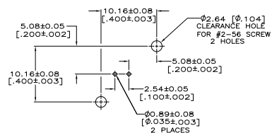
PCB CONFIGURATION
