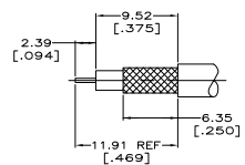
RECOMMENDED STRIP LENGTH SCALE 4:1
