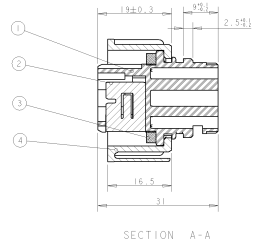
SECTION A-A SECOND LOCKING DEVICE IN PRE-LOCKED POSITION
