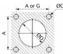
Front mounting
